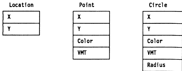
Figure 5.1 shows layouts of instances of Location , Point , and Circle ; each box corresponds to one word of storage.
